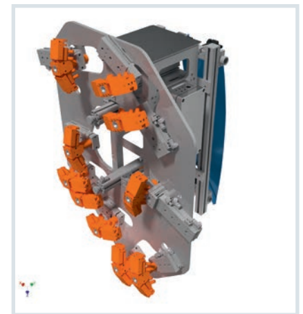
Fig. 5. Wrinkle-free production: the ten separate, individually movable needle grippers (orange) and eleven strokes allow for safe insertion and clamping of the decoration of the A-pillar finisher (© KraussMaffei)
